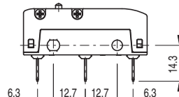
Terminali a faston H verticali
